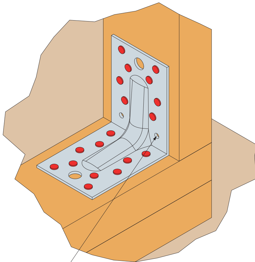
NAIL PATTERN (E2/2.5/7090)
